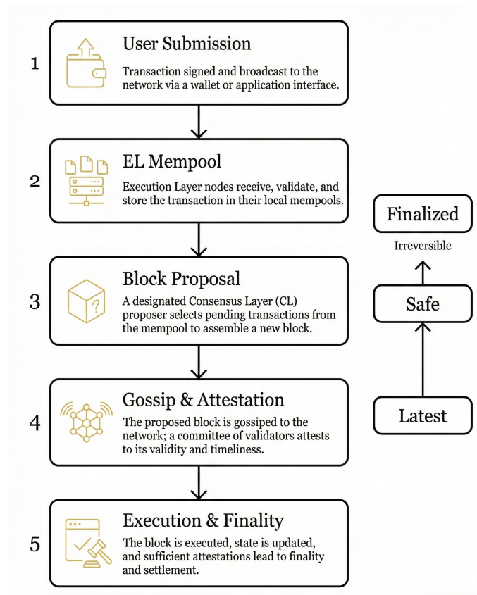
Figure 3: Transaction Lifecycle — From Submission to Finality
