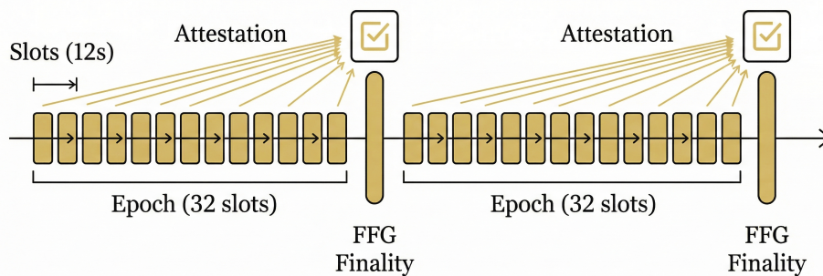
Figure 2: Epoch Structure with Attestations and FFG Finality
