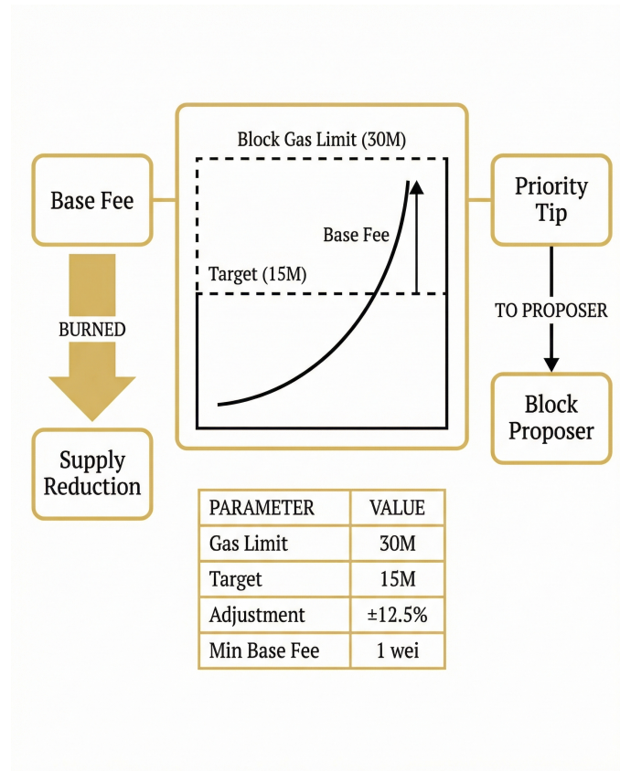
Figure 4: EIP-1559 Fee Mechanism and Gas Parameters
